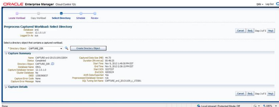
FIGURE 9.51 The Preprocess Captured Workload: Select Directory screen
